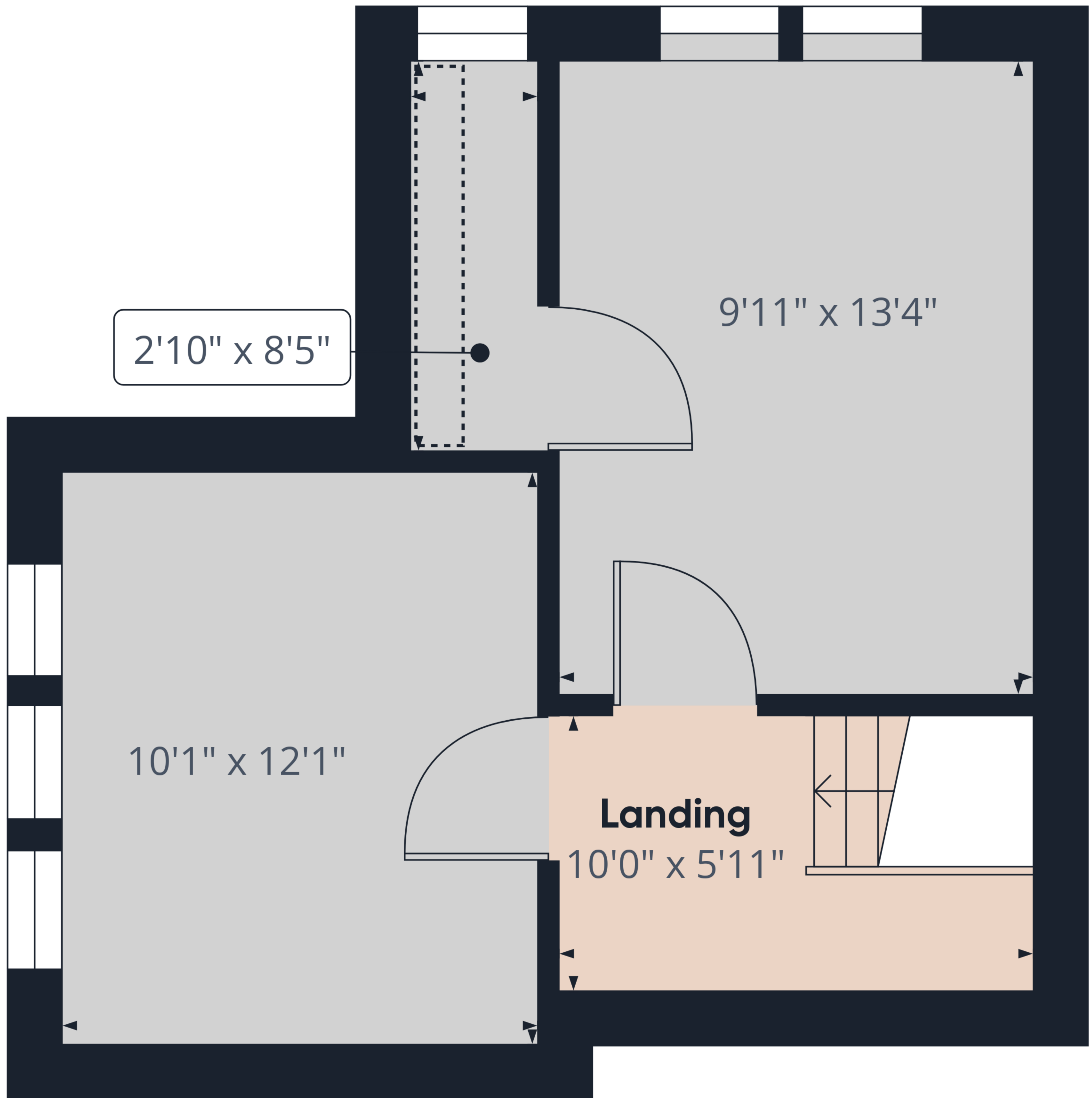
Floor 1
