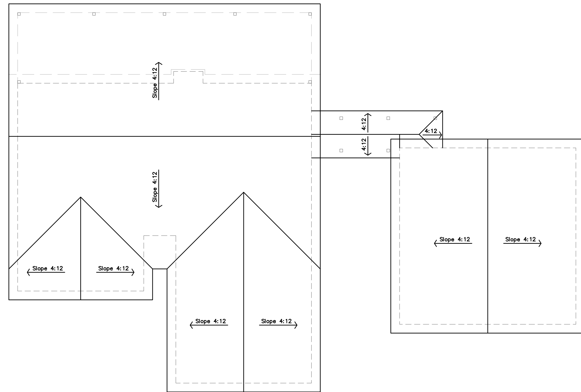
B ROOF PLAN 1/8"=0"
