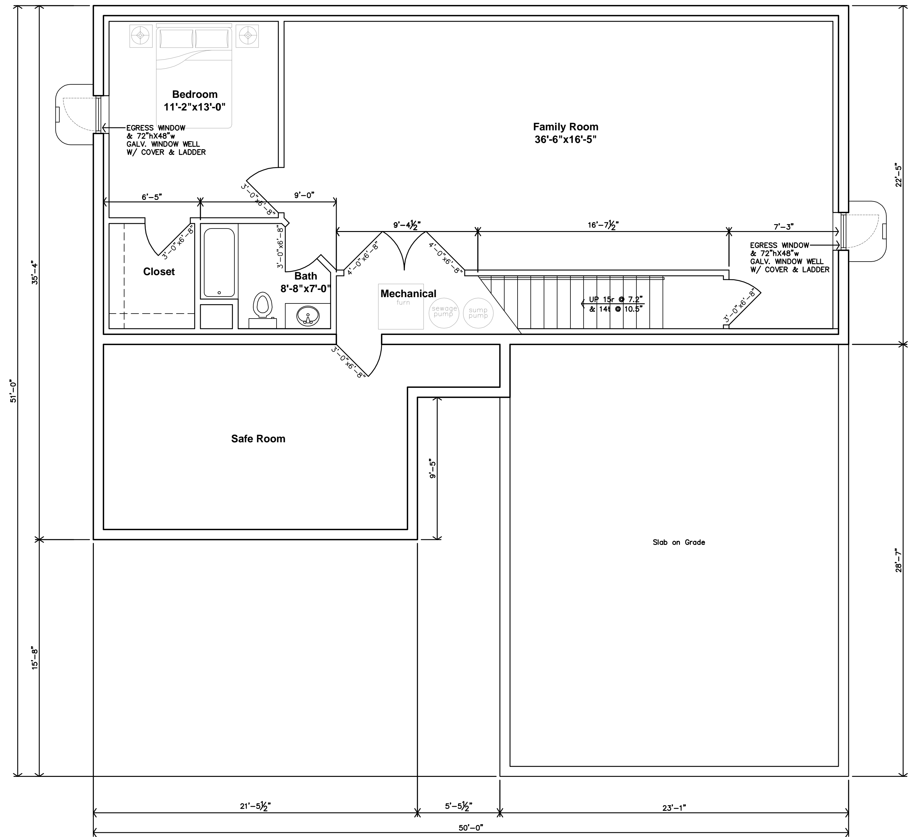
A BASEMENT FLOOR PLAN 1/4"=1'-0"
